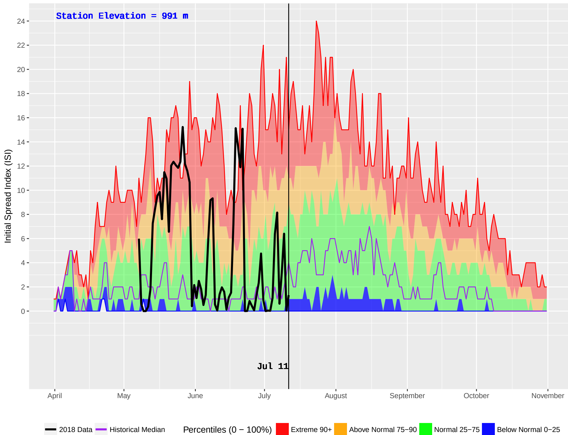
TROUT LAKE (387) : Historical (1987–2016) and Current (2018) Noon Initial Spread Index (ISI)
