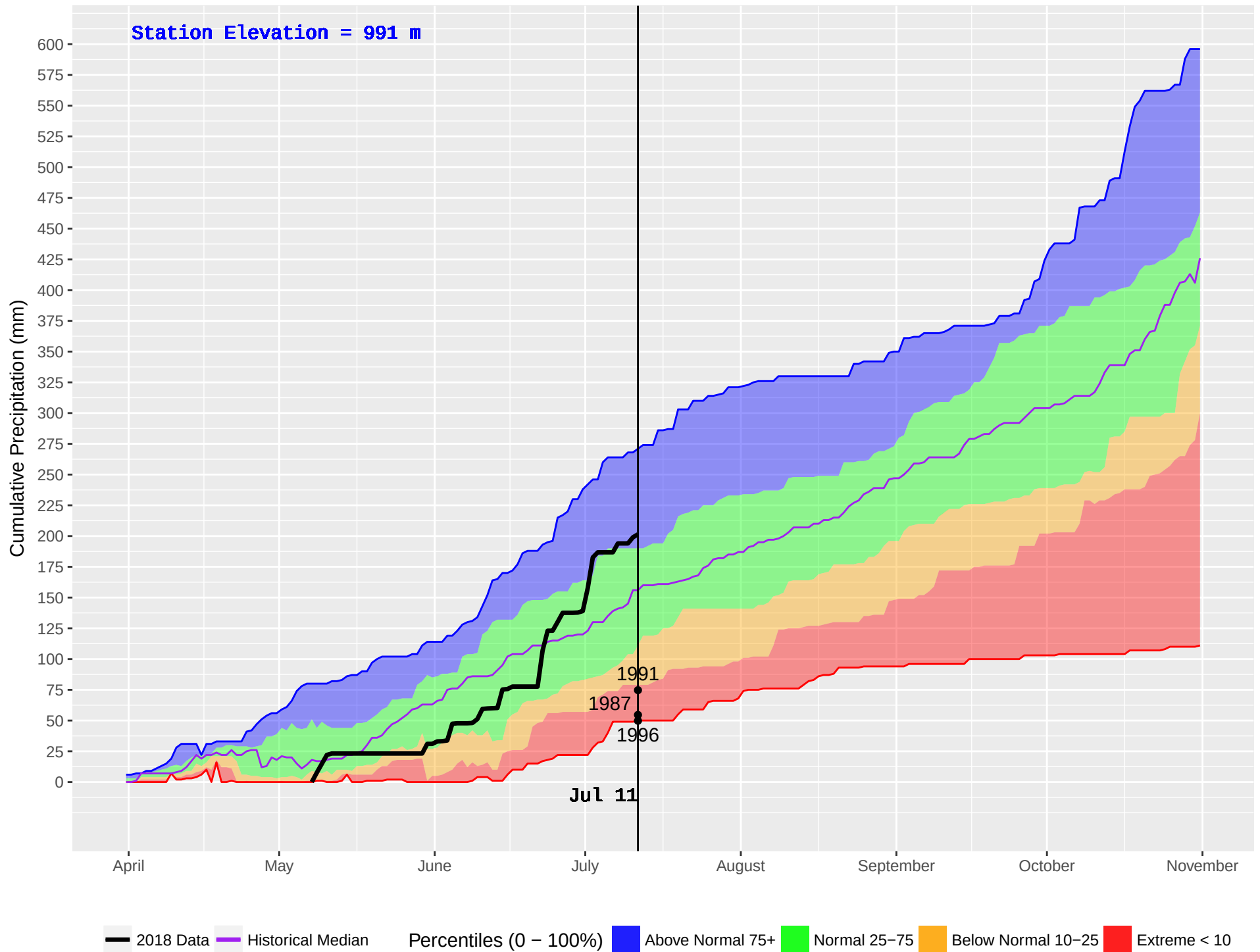
TROUT LAKE (387) : Historical (1987–2016) and Current (2018) Noon Cumulative Precipitation
