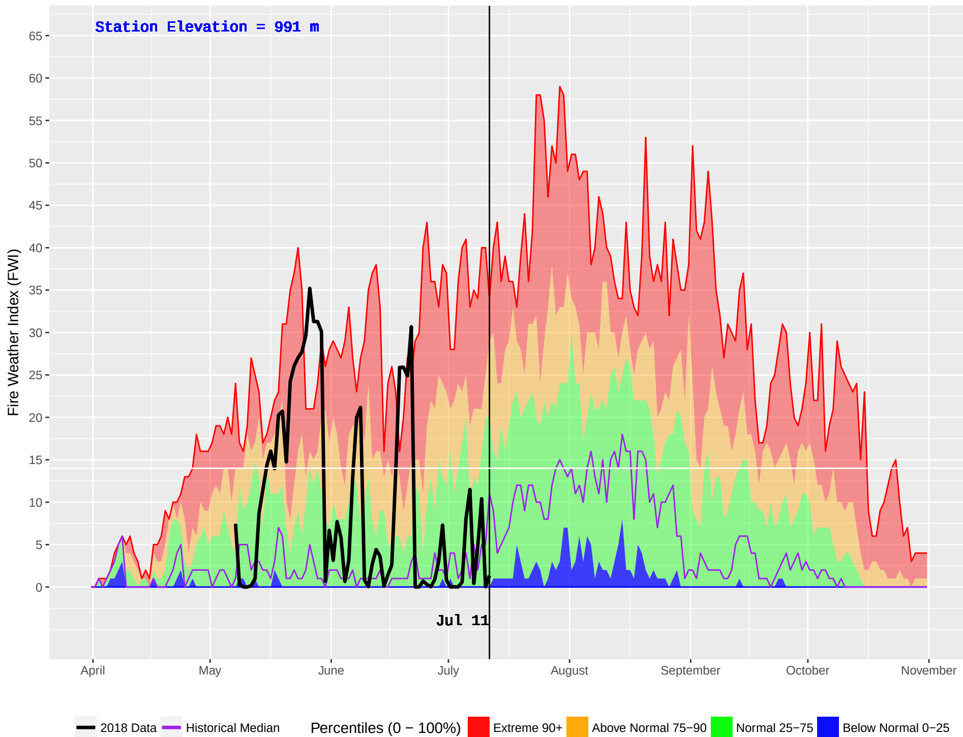
TROUT LAKE (387) : Historical (1987–2016) and Current (2018) Noon Fire Weather Index (FWI)
