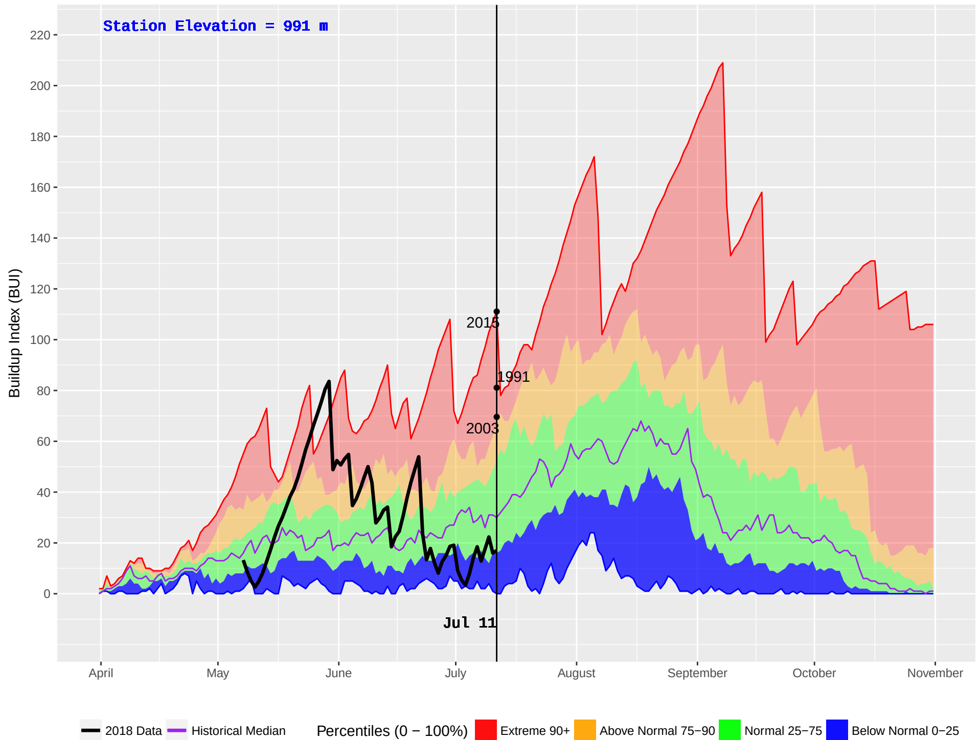
TROUT LAKE (387) : Historical (1987–2016) and Current (2018) Noon Buildup Index (BUI)
