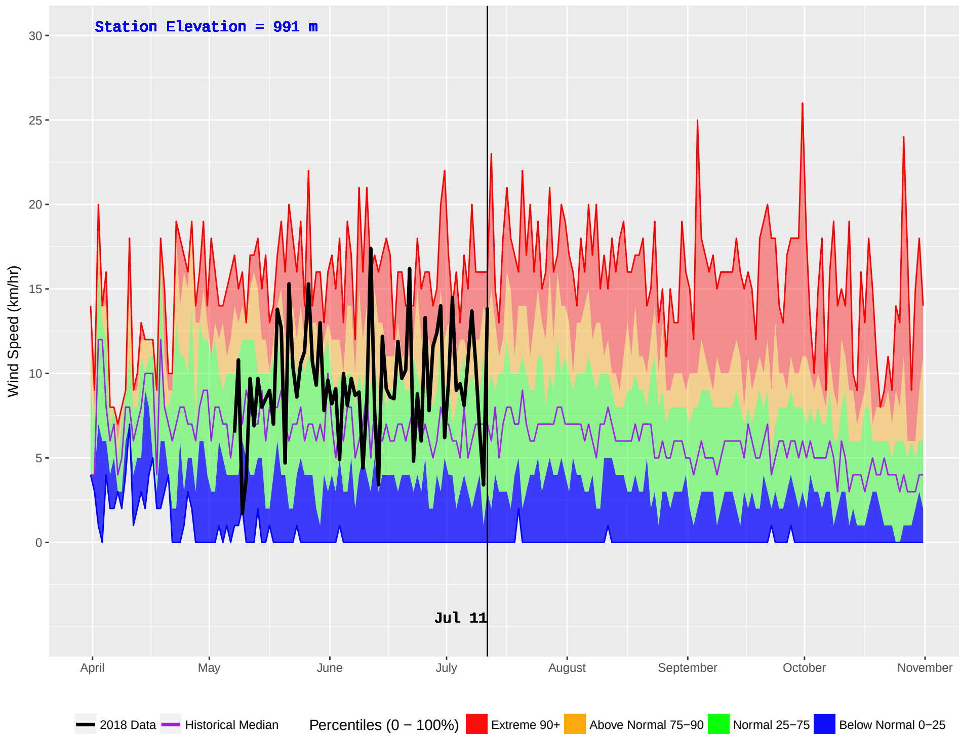
TROUT LAKE (387) : Historical (1987–2016) and Current (2018) Noon Wind Speed
