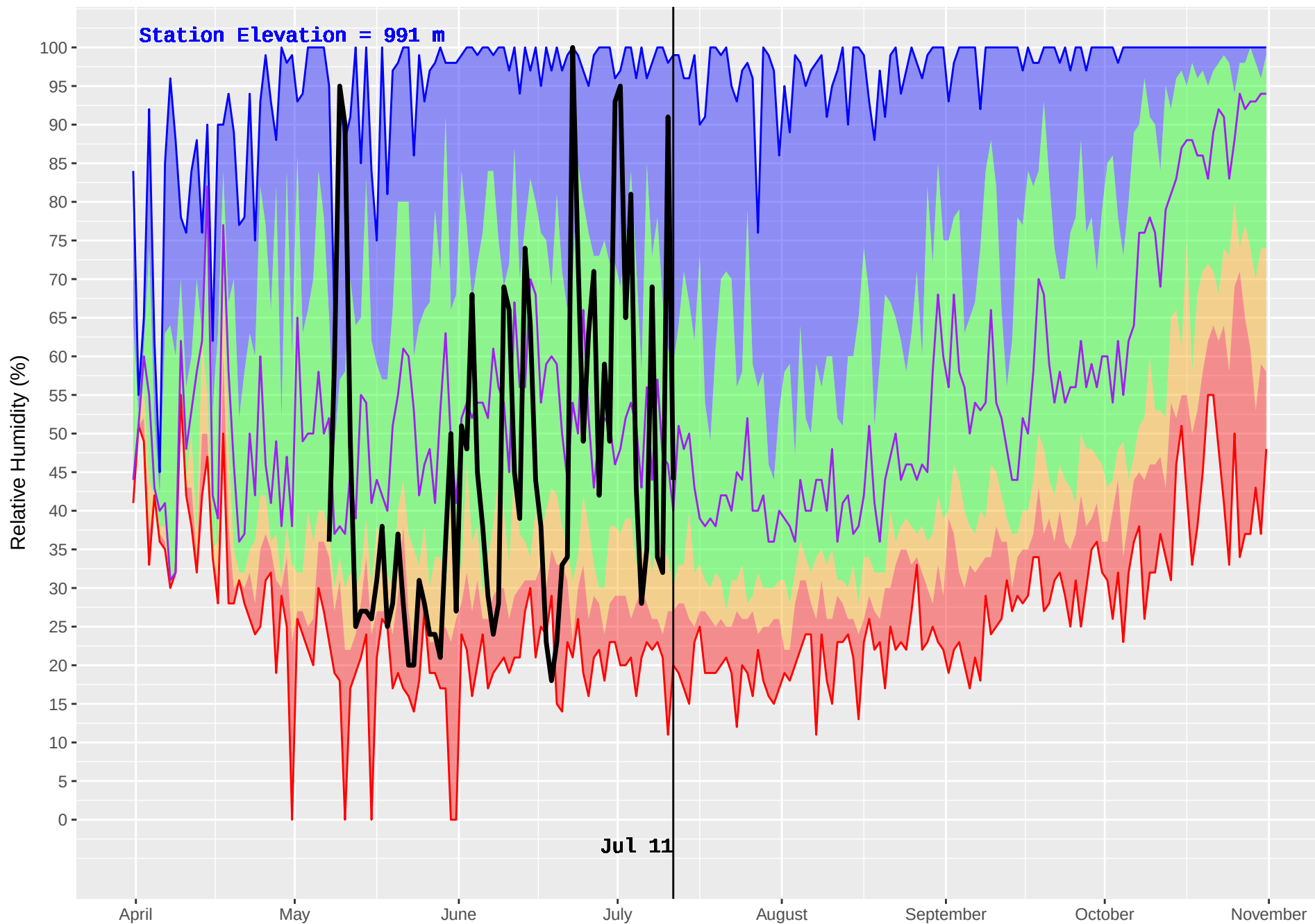
TROUT LAKE (387) : Historical (1987–2016) and Current (2018) Noon Relative Humidity
