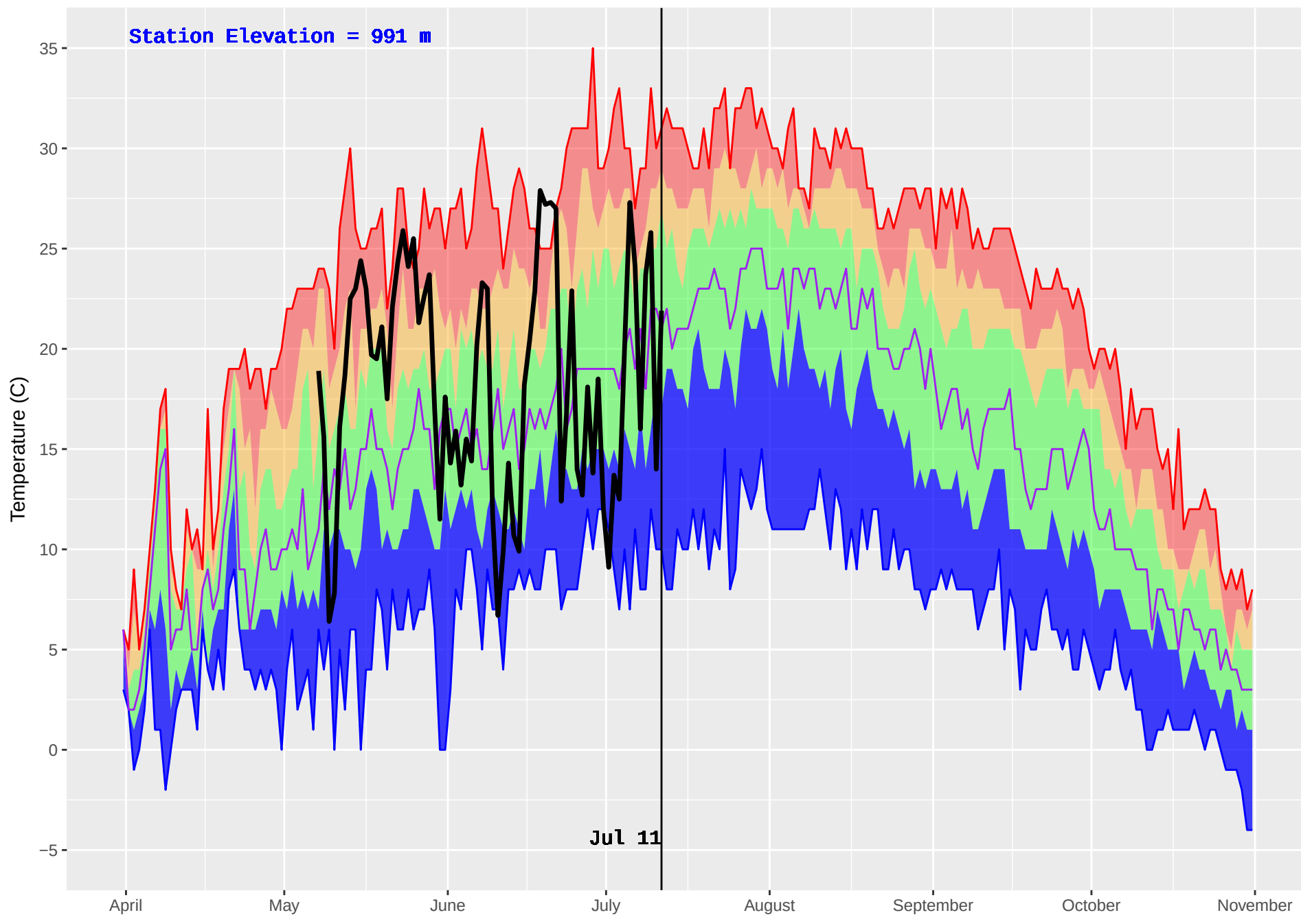
TROUT LAKE (387) : Historical (1987–2016) and Current (2018) Noon Temperature
