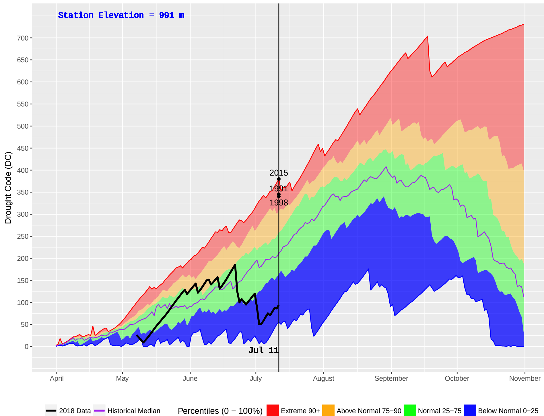
TROUT LAKE (387) : Historical (1987–2016) and Current (2018) Noon Drought Code (DC)
